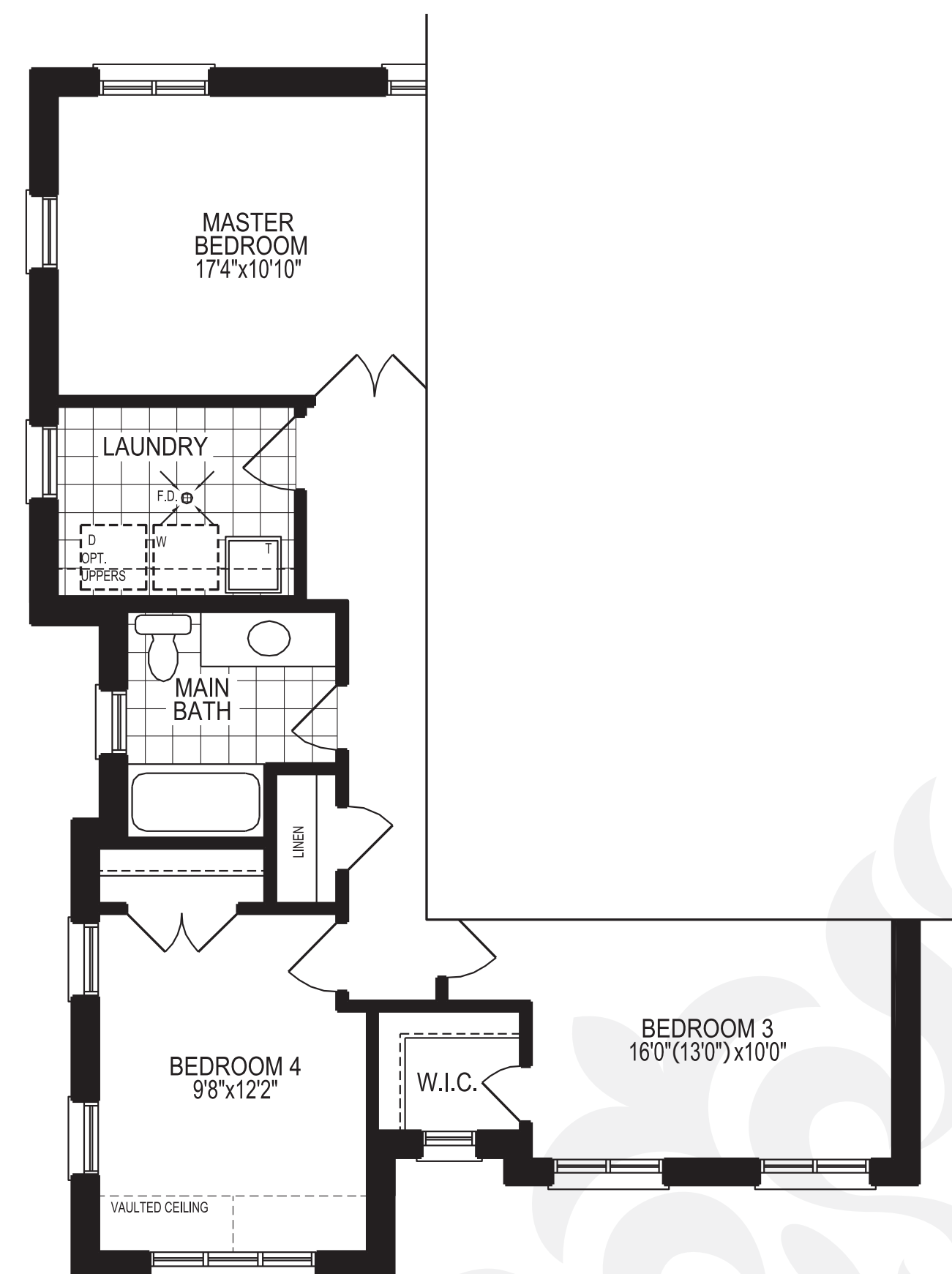
PARTIAL SECOND FLOOR EL. 'B'
