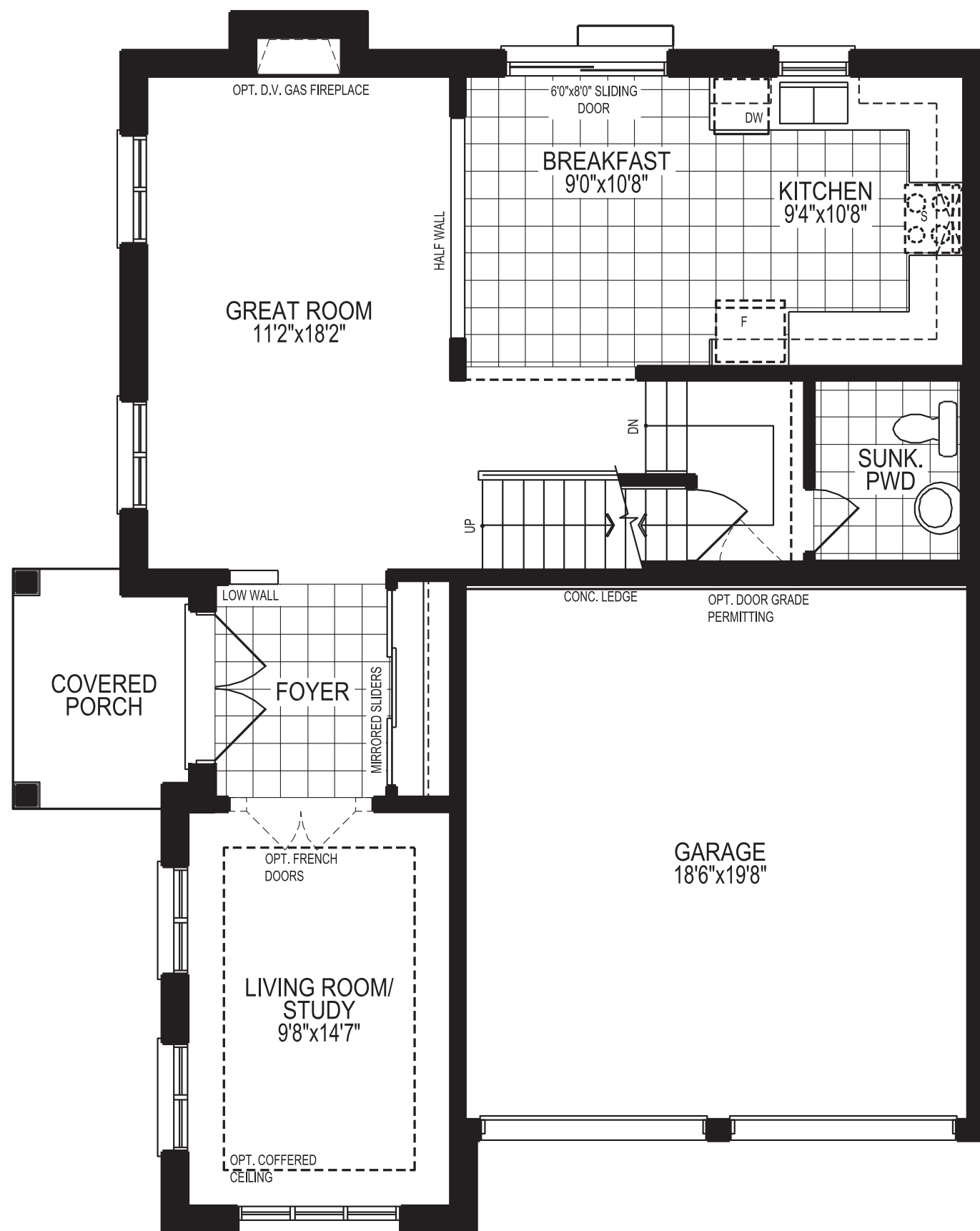
GROUND FLOOR EL. 'A'
