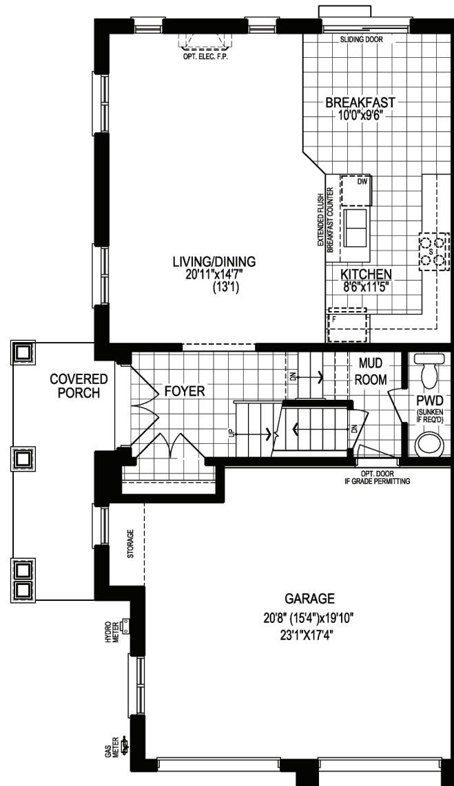
GROUND FLOOR PLAN, EL. 'B' (FOR LOTS 1 & 107 ONLY)
