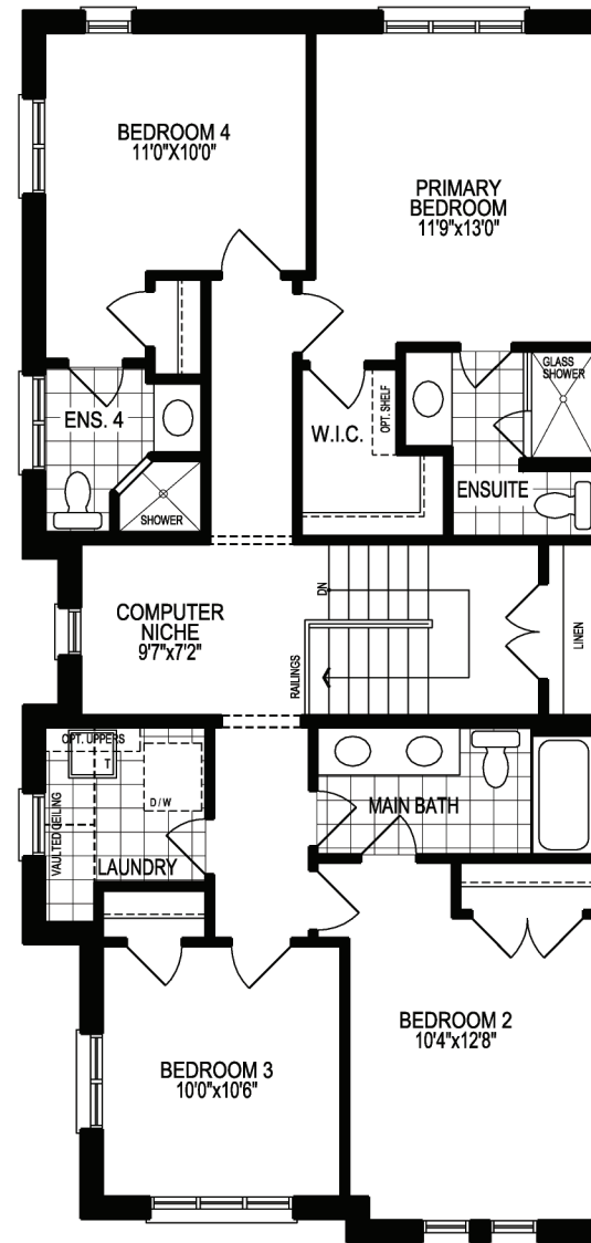
SECOND FLOOR PLAN, EL. 'B' (FOR LOTS 1 & 107 ONLY)
