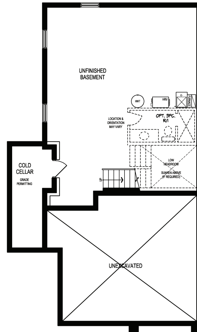
BASEMENT PLAN, EL. 'B' (FOR LOTS 1 & 107 ONLY)
