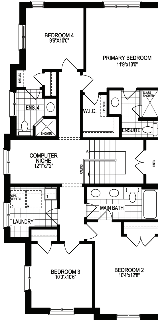
SECOND FLOOR PLAN, EL. 'A' (FOR LOTS 90, 91, & 108 ONLY)
