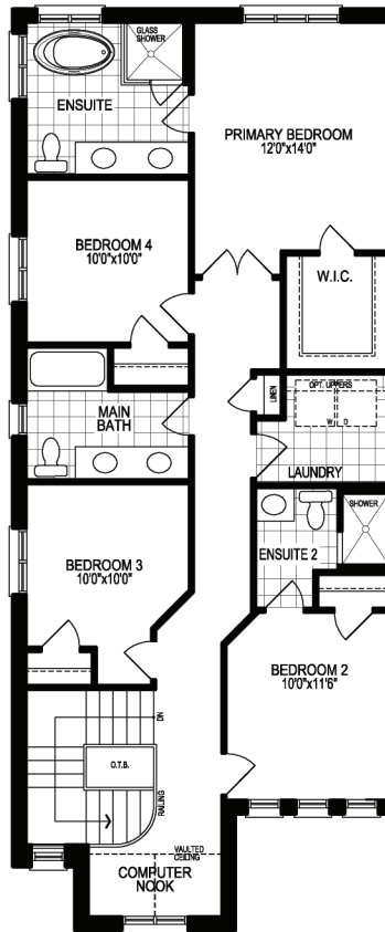
SECOND FLOOR PLAN, EL. 'A1'
