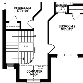
SECOND FLOOR PLAN, EL. 'B1'
