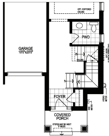
GROUND FLOOR PLAN, EL. 'A2' & 'B2' (REV)
