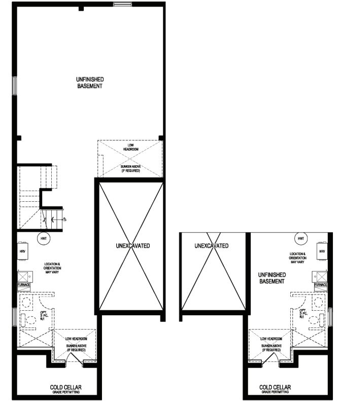
BASEMENT PLAN, EL. 'A1'
