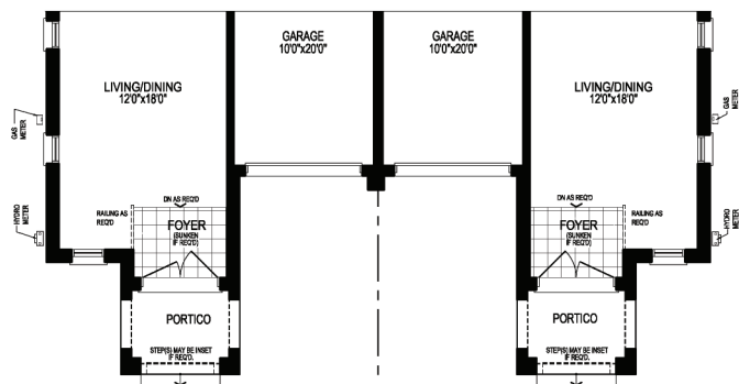
GROUND FLOOR PLAN, EL. 'B1'
