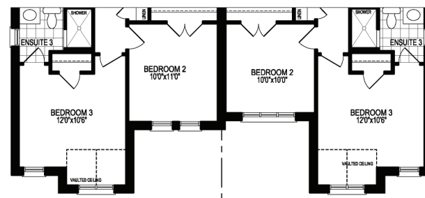
SECOND FLOOR PLAN, EL. 'B1'
