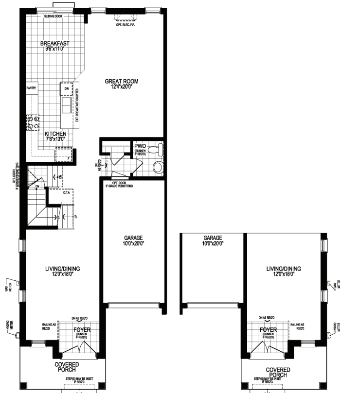
GROUND FLOOR PLAN, EL. 'A1'
