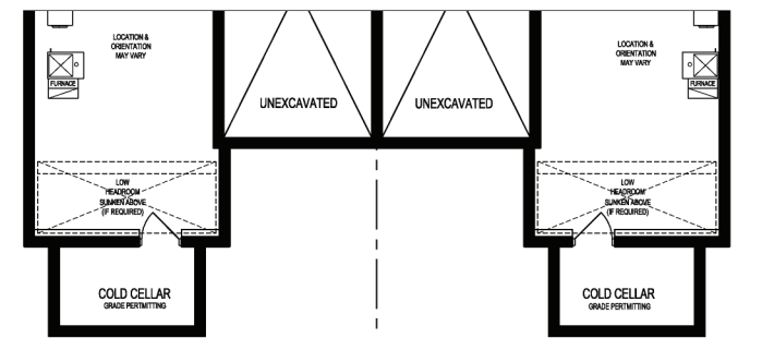
BASEMENT PLAN, EL. 'B1'
