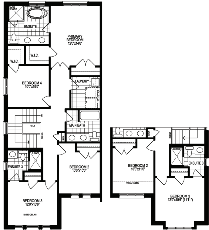
SECOND FLOOR PLAN, EL. 'A1'
