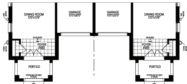
GROUND FLOOR PLAN, EL. 'B1'
