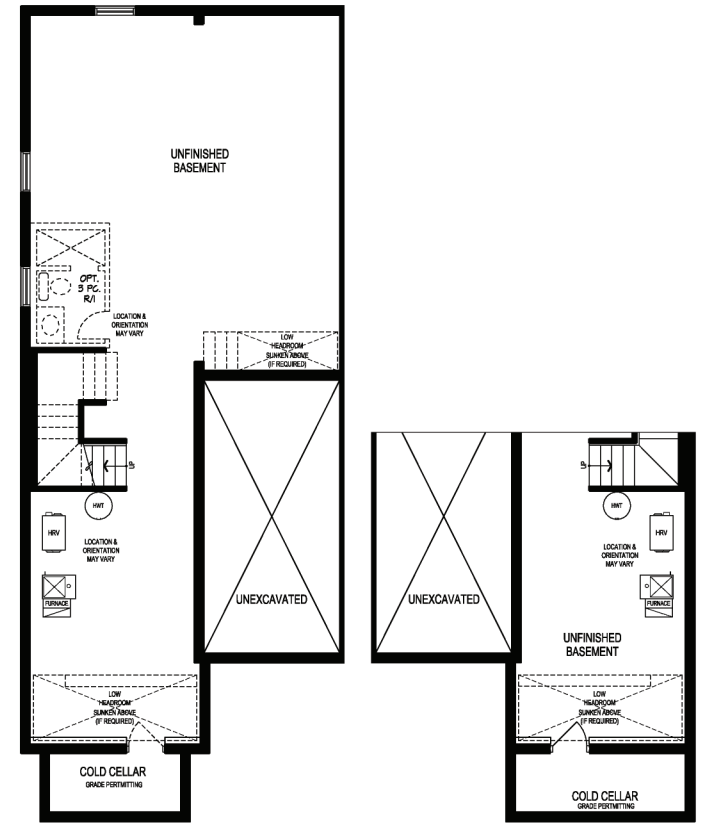
BASEMENT PLAN, EL. 'A1'
