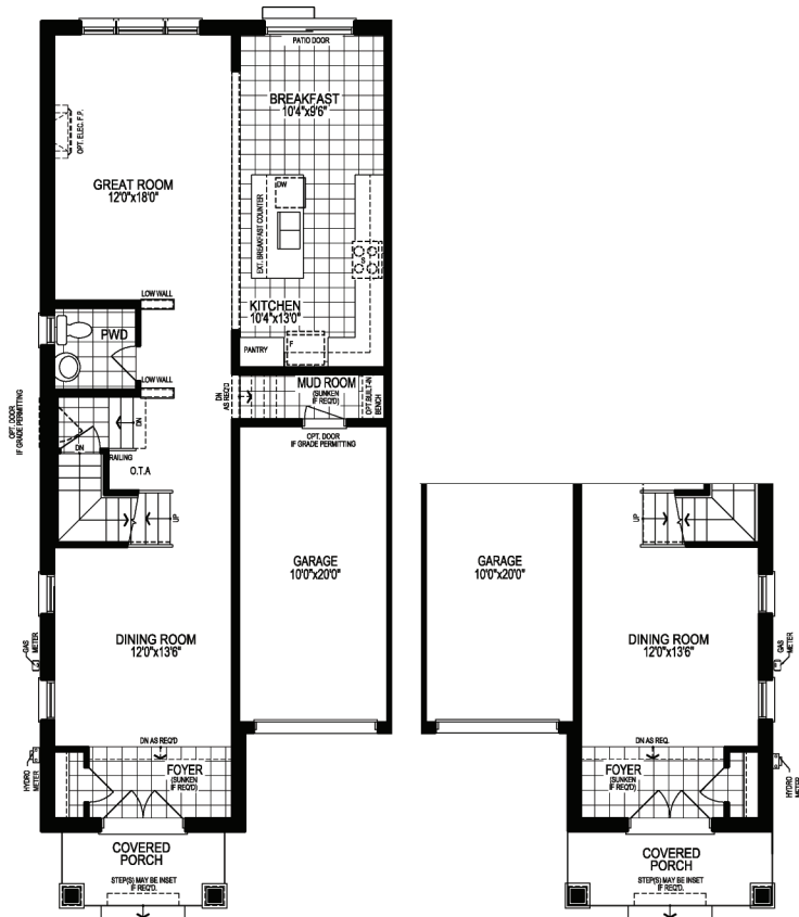
GROUND FLOOR PLAN, EL. 'A1'
