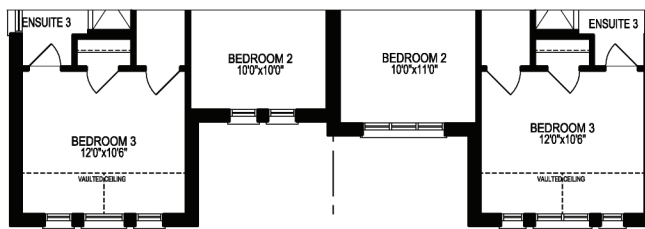
SECOND FLOOR PLAN, EL. 'B1'
