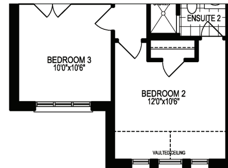
SECOND FLOOR PLAN, EL. 'B'
